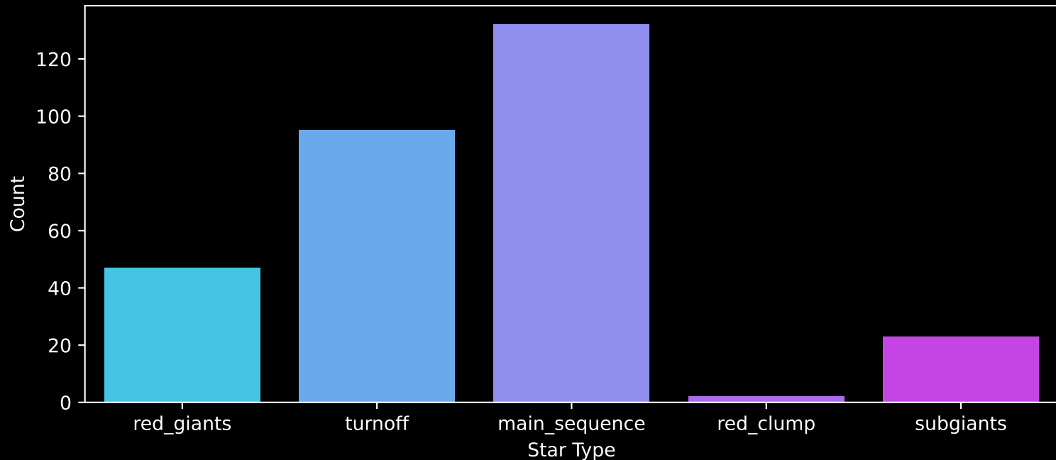
GALAH DR4 Field: [453] Count plot of Star Type
