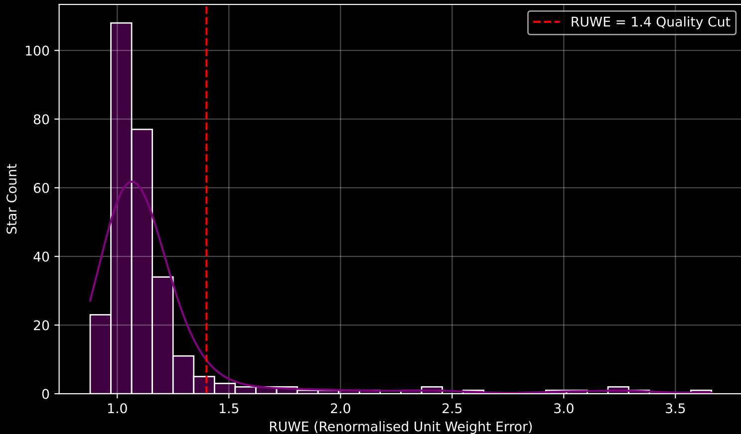
GALAH DR4 Field [453] RUWE Distribution (n= 281)
