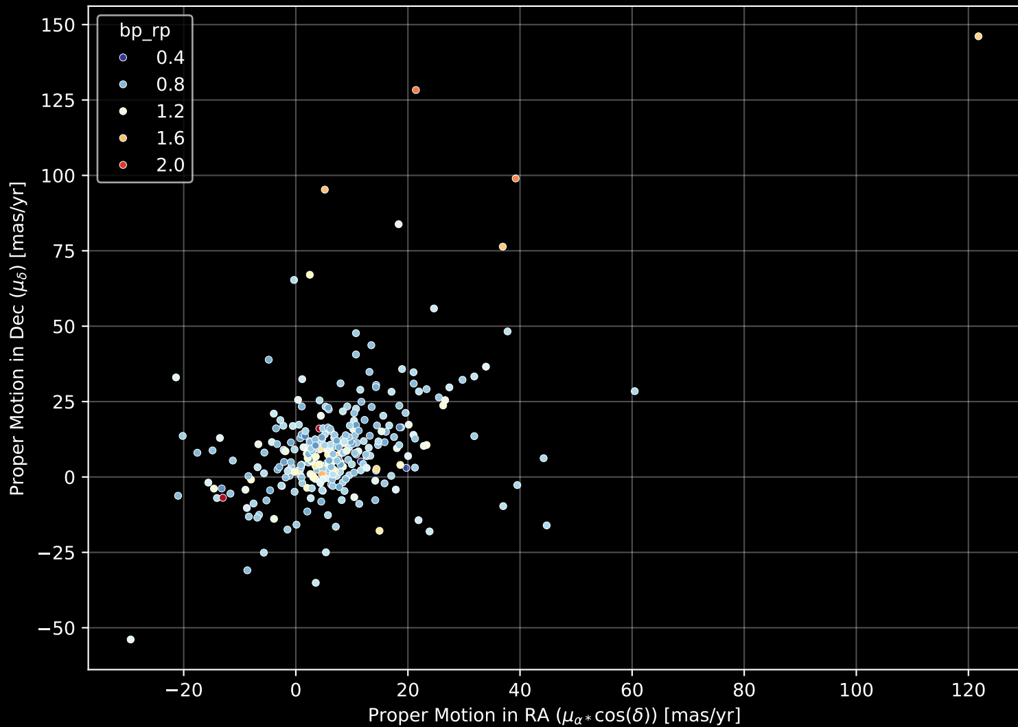
GALAH DR4 Field: [453] Proper Motion Diagram (n= 299)
