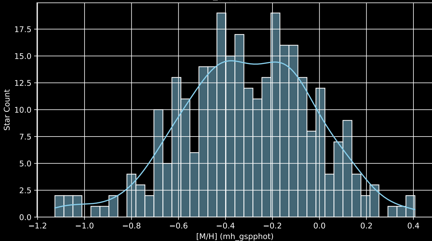
GALAH DR4 Field: [453] [M/H] (mh_gspphot) (n= 296)
