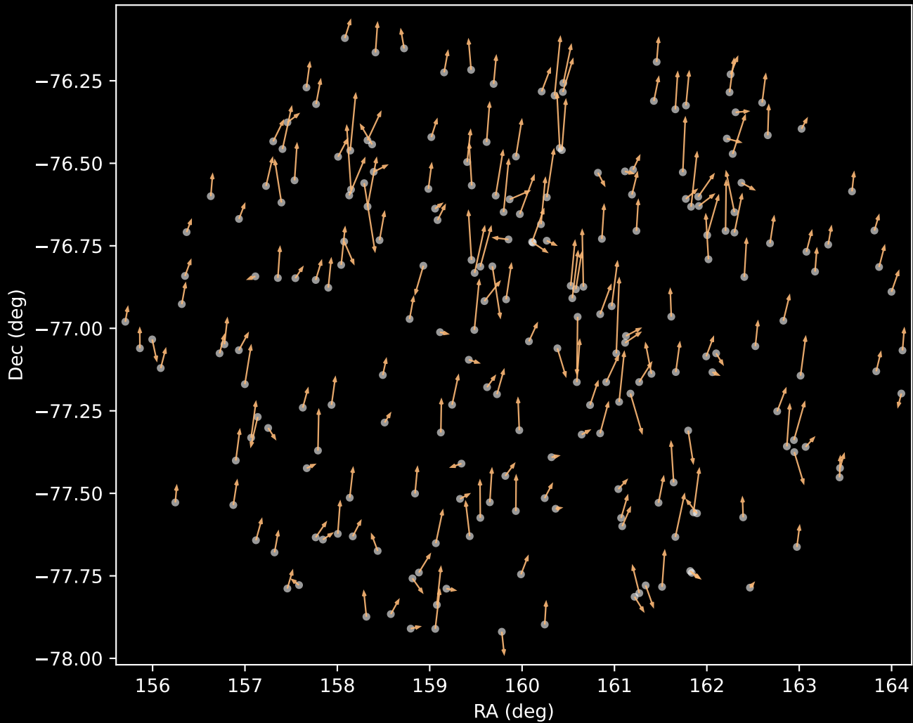
GALAH DR4 Cluster 3 Proper Motion Vectors (n=224)
